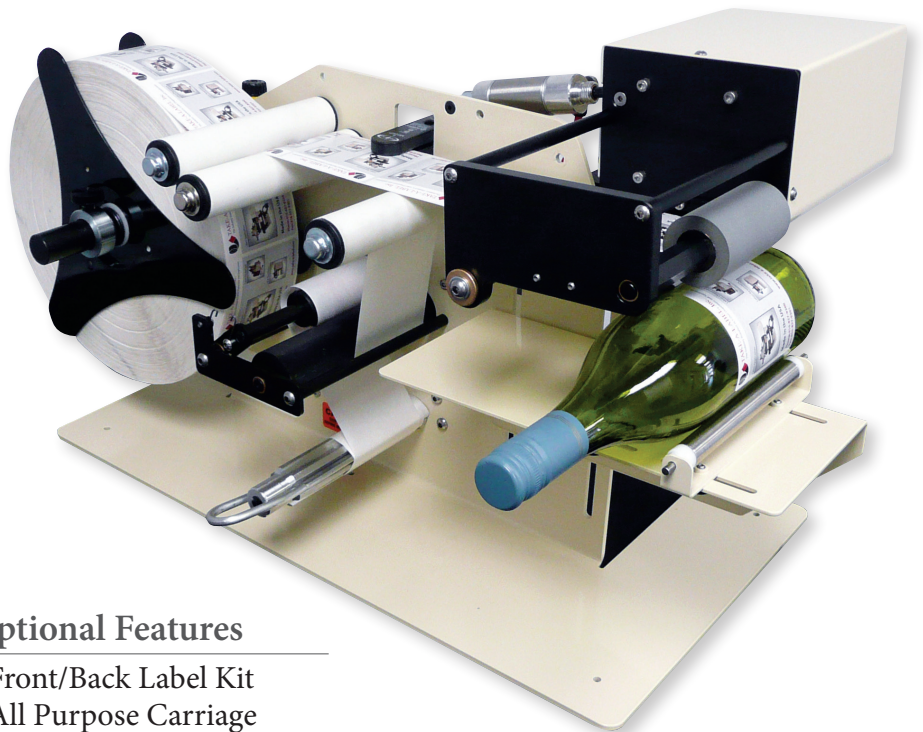
Model TAL-3100R Applicator
